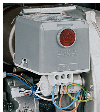
Control box fitted with an ignition transformer
