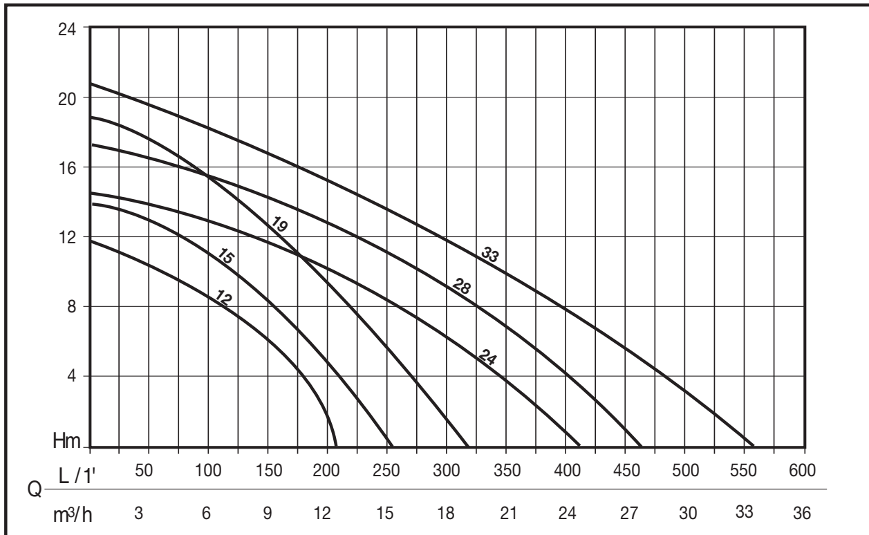
PUMP PERFORMANCE
